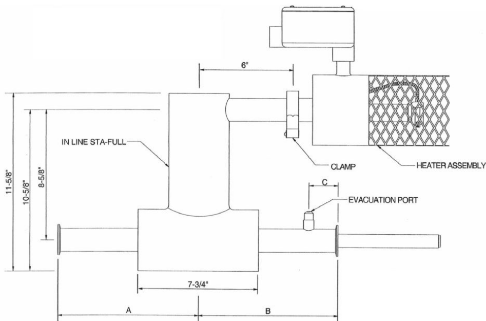
StatiFlex / DynaFlex Dimensions
