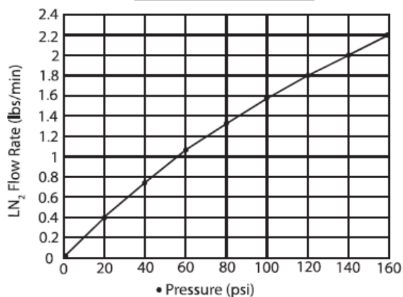
CRYOVENT FLOW RATE
